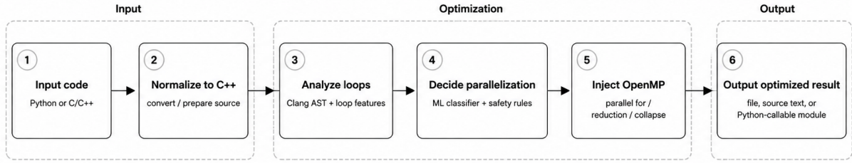
Figure 3.3: Code Parallelizer module workflow
