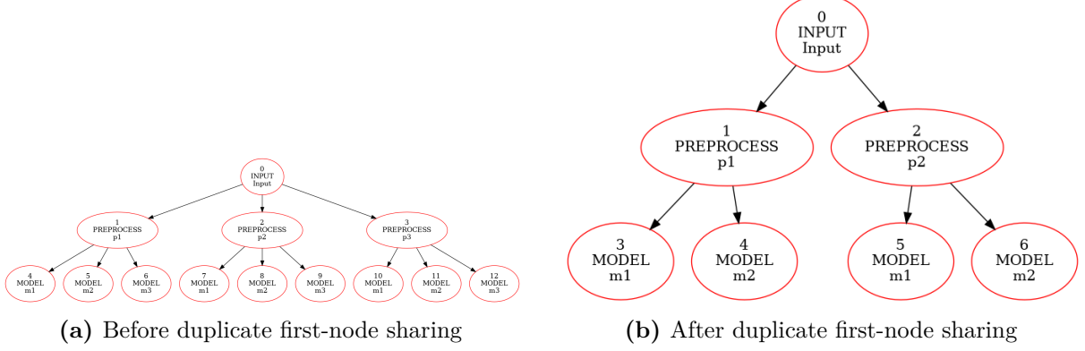
Figure 3.2: Branch graph before and after sharing equivalent first branch nodes.
